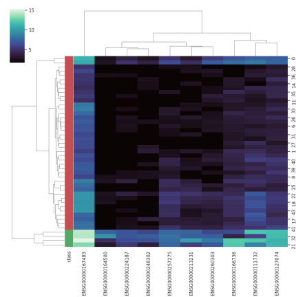
(c) HeatMap GSE68799 - Top 10 Genes
